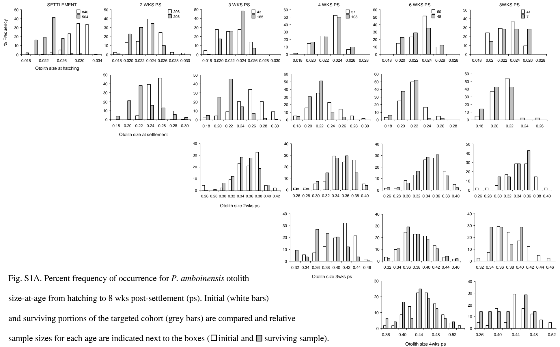
Fig. S1. Frequency distribution of selected otolith-derived traits of P. amboinensis from hatching to 8 weeks post-settlement.
