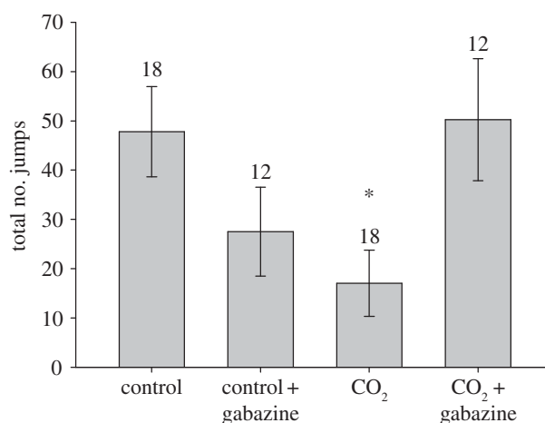
Figure 4. The total number of jumps per individual in control or elevated- \text{CO}_2 snails treated with a seawater sham or gabazine, and then exposed to predator cue. In elevated- \text{CO}_2 snails, jumping behaviour was restored by gabazine. Values are means \pm s.e. Numbers of replicates are given above the bars. Asterisk (*) denotes a significant difference from control.
